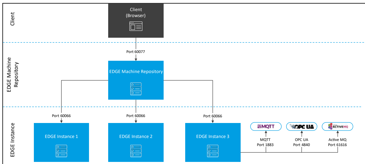
Fig. 2: Communication of FORCAM FORCE Machine Repository with EDGE Config. and paths
